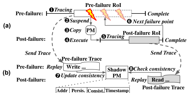
Figure 8. XFDetector’s (a) frontend and (b) backend.
