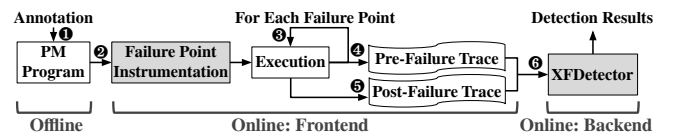
Figure 7. An overview of XFDetector.
