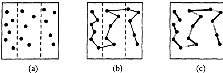
Figure 5.12 (a) Partitioning a net into strips/chains; (b) a serpentine tour with low density, low average cost, and low density; and (c) an embedded geometric matching which also has low density and low average cost.
