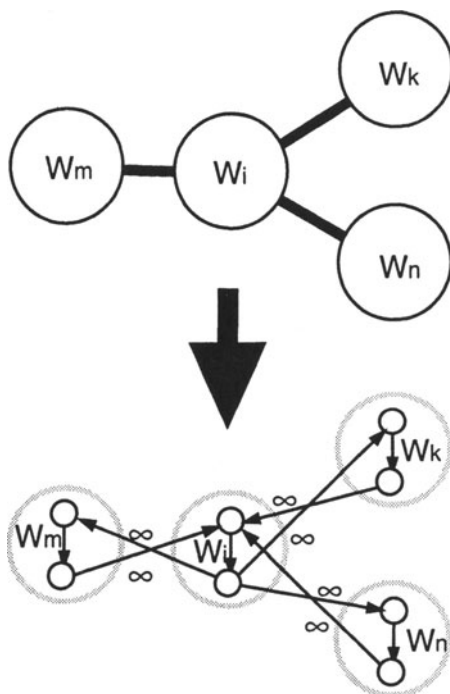
Figure 5.23 Transformation of a node- and arc-capacitated flow network to an arc-capacitated flow network: arc capacities c_{ij} remain infinite, while original node capacities (node weights) c_i^i induce directed arc capacities in the transformed network.
