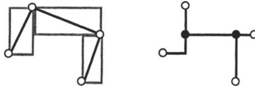
Figure 2.5 Optimal overlap of MST edges within their bounding boxes.
