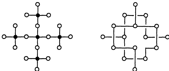
Figure 2.6 Example with strict equality \frac{\text{cost}(\text{MST-Overlap})}{\text{cost}(\text{SMT})} = \frac{3}{2} . On the left is the SMT ( \text{cost} = 20 ); any Steiner tree derived from the MST on the right will have \text{cost} = 30 .
