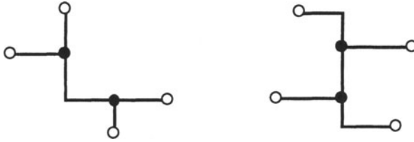
Figure 2.15 The two possible Steiner tree topologies on 4 points.
