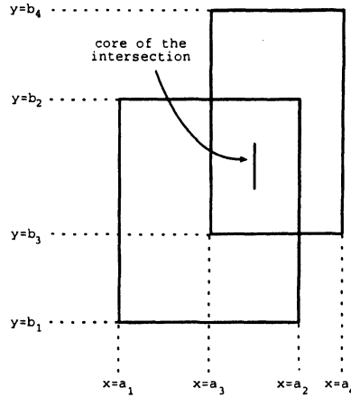
Figure 4.14 Intersecting two TRRs after 45-degree rotation.
