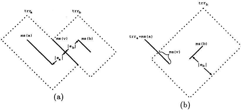
Figure 4.12 Two cases in construction of merging segment ms(v) . (a) Merging cost equals \kappa = d(ms(a), ms(b)) . (b) Merging cost is greater than \kappa (note that in this example radius(trr_a) = |e_a| = 0 ).
