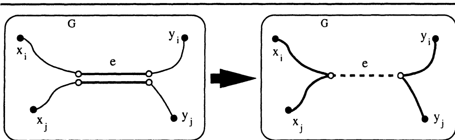
Figure 4.6 An edge can belong to at most one shortest path in an optimal complete generalized matching.
