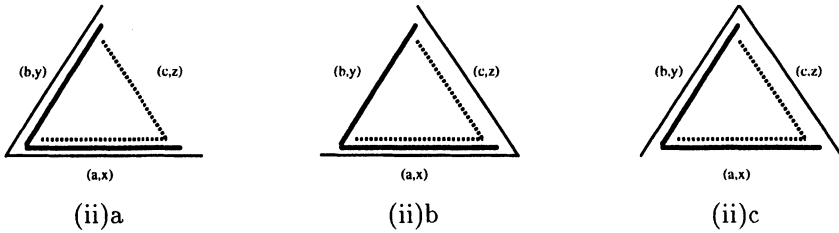
Figure 5.17 Topology of the three spanning trees MST(G_2) (inner), MST(G_1) (middle) and MST(\widehat{G}(\vec{d})) (outer) corresponding to case (ii)a, case (ii)b, and (ii)c.
