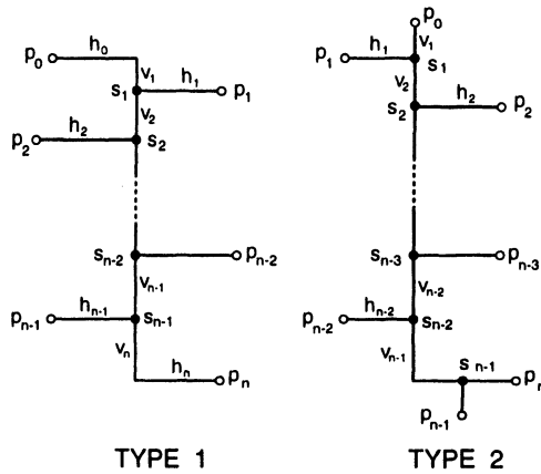
Figure 2.3 Two types of SMTs in M_1 : Type 1 has all of its Steiner points on a line; Type 2 has all but one of its Steiner points on a line.
