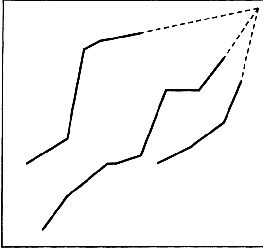
Figure 5.11 Combining chains into a low-density tree.
