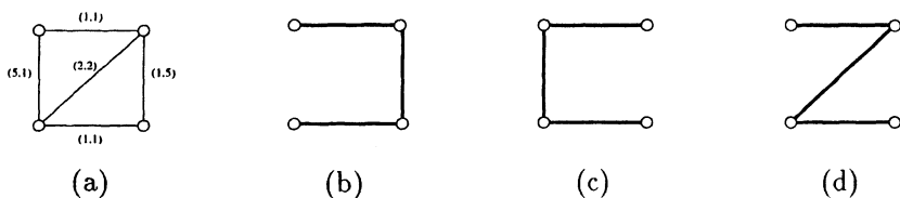
Figure 5.13 (a) A 2-weighted graph G , and MSTs over its two induced graphs: (b) \text{MST}(\widehat{G}((1, 0))) with cost 3 + 7 = 10 , and (c) \text{MST}(\widehat{G}((0, 1))) with cost 7 + 3 = 10 ; (d) shows the MST over the tradeoff graph: \text{MST}(\widehat{G}((\frac{1}{2}, \frac{1}{2}))) with cost 4 + 4 = 8 .
