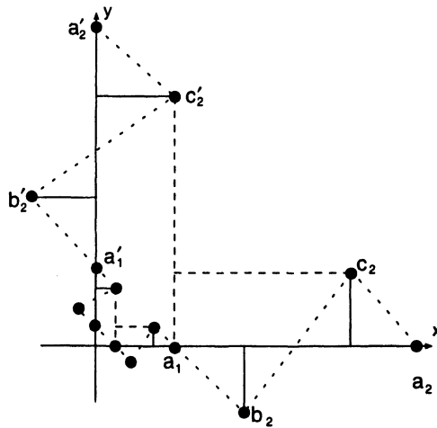
Figure 2.19 The construction of Berman et al. which establishes a lower bound of 1.3 on the IIS performance ratio.
