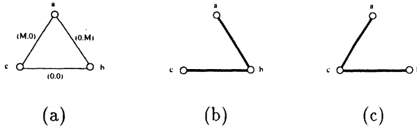
Figure 5.14 An example showing that \overline{\text{MST}}(\widehat{G}(\vec{d})) cannot be bounded from above by any function strictly in terms of \overline{\text{MST}}(G_i) 's, \vec{d} , n , and k : (a) The 2-weighted graph G ; (b) \text{MST}(G((1, 0))) has cost 0; (c) \text{MST}(G((0, 1))) has cost 0. On the other hand, \text{MST}(G((\frac{1}{2}, \frac{1}{2}))) has cost \frac{M}{2} , which can be arbitrarily large.
