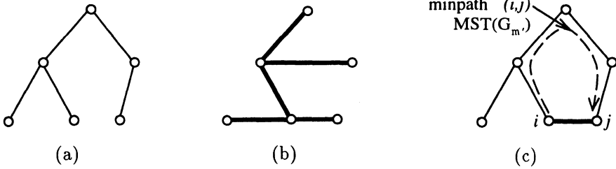
Figure 5.15 A general upper bound in the metric case: for \overline{\text{MST}}(\widehat{G}(\vec{d})) in terms of \overline{\text{MST}}(G_i) 's, \vec{d} , n , and k : (a) depicts \text{MST}(G_m) ; (b) depicts \text{MST}(\widehat{G}(\vec{d})) ; and (c) shows how the cost of the m^{\text{th}} weight component of each e_{ij} can be bounded by d_m \cdot \overline{\text{MST}}(G_m) .
