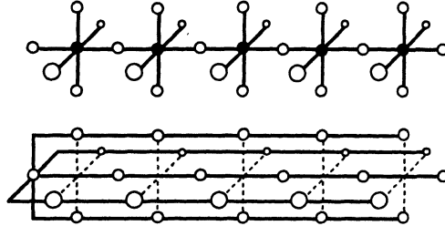
Figure 2.9 For d = 3 , the SMT (top) has cost \frac{6}{5}(n - 1) , while any Steiner tree derivable from the MST by re-embedding edges (bottom) has cost 2(n - 3) , yielding performance ratio arbitrarily close to \frac{5}{3} as n grows large.
