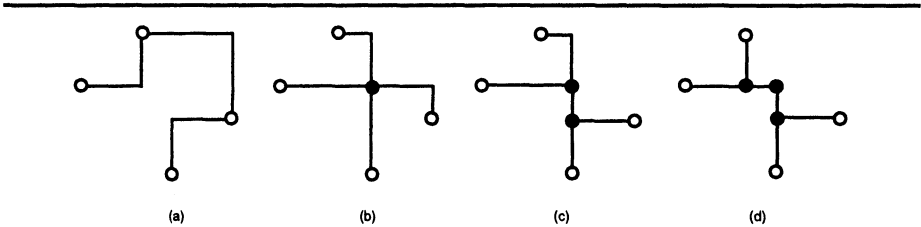
Figure 2.11 Example of the execution of Iterated 1-Steiner (I1S). Note that in step (d) a degree-2 Steiner point results; I1S will eliminate this point from the topology.
