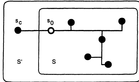
Figure 3.24 The CSRT problem with a single critical sink is NP-hard for any choice of technology parameters. A rectilinear SMT instance S is transformed into a CSRT instance S' = S \cup \{s_c\} which has critical sink s_c directly left of s_0 \in S which has smallest x -coordinate. The optimal CSRT solution consists of a rectilinear SMT over S , plus the edge (s_0, s_c) .
