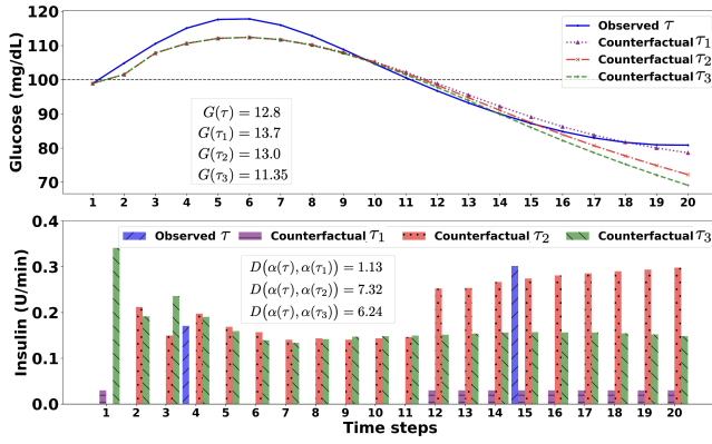
Figure 1: Observed and counterfactual trajectories of glucose levels (states) and insulin dosages (actions) over one hour.
