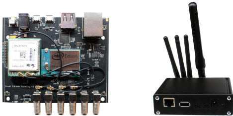
Fig. 4: Gateway hardware. The gateway contains a dedicated radio for receiving Triumvi packets and additional radios (WiFi, BLE, and cellular) for transmitting the data.
