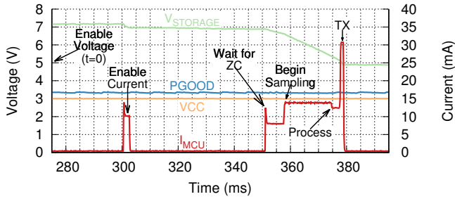
Fig. 7: Current and voltage trace of a Triumvi measurement. The voltage on the storage capacitor, PGOOD, VCC, and the current draw of the microcontroller are shown while Triumvi measures power. At the start (not shown) Triumvi enables the voltage measurement circuit and waits 300 ms. It then enables the current measurement circuit before waiting for a rising zero-crossing of the AC voltage signal to start sampling the current for 16.6 ms. After, it computes power, encrypts, and transmits the measurement.
