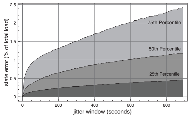
Figure 6: Impact of jitter on state error
