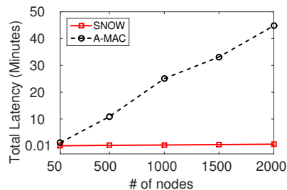
(a) Latency for convergecast
