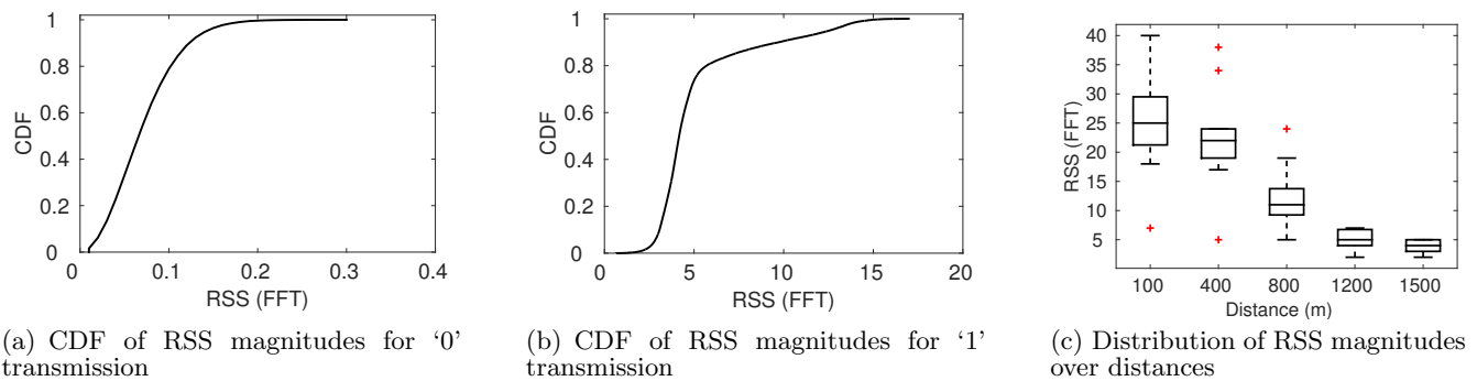
Figure 3: Threshold behavior
