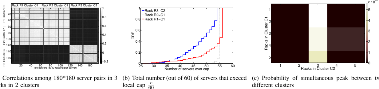
Fig. 8. Correlations among servers, racks, and clusters
