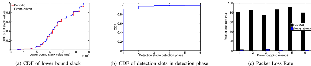
Fig. 9. Performance of Event-Driven protocol on 60 servers (4 weeks)
