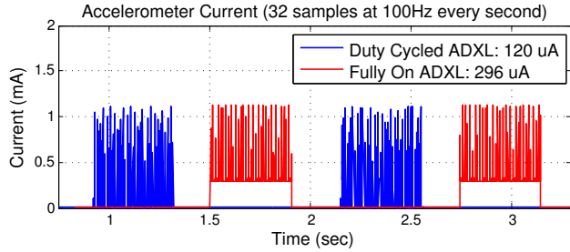
Figure 16: Current consumption of an ADXL335 3-axis analog accelerometer, sampling 32 bytes every second at 100 Hz. Current for a constantly on ADXL335 vs. one that is power-gated ('Duty Cycled') are shown, offset in phase for clarity. Power-gating reduces average current consumption from 296 \mu\text{A} to 120 \mu\text{A} .
