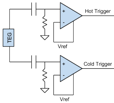
Figure 5: Comparator-based low power wakeup trigger. Hot Trigger or Cold Trigger will activate when there is any small deviation in \Delta T , indicating water flow.
