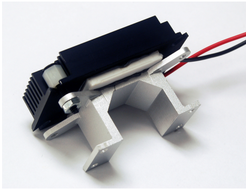
Figure 3: Peltier module including aluminum thermal coupler and heatsink. Four arms extend to fasten a heatsink to the Peltier module and coupler. The 0.75”-wide octagonal portion is covered in thermal compound prior to attachment to a right angle valve.
