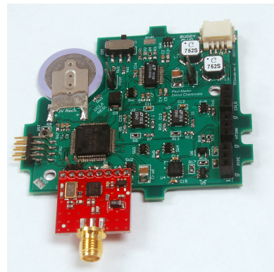
Figure 10: DoubleDip node—ultra low power energy harvesting node with low latency wakeup, pipe vibration sensing, temperature sensors, and RF. The board size is roughly 3 \times 3 in.
