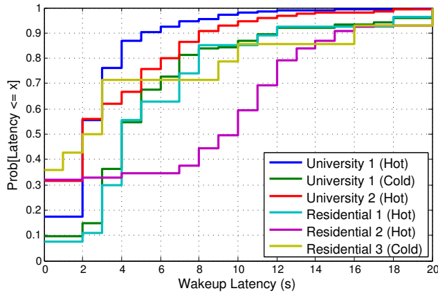
Figure 14: Cumulative distribution function (CDF) for wakeup latencies across all nodes.
