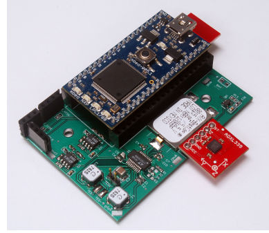
Figure 9: Testing PCB for 24/7 fine-grained monitoring of temperatures, accelerations, and energy harvested from both hot and cold water pipes.
