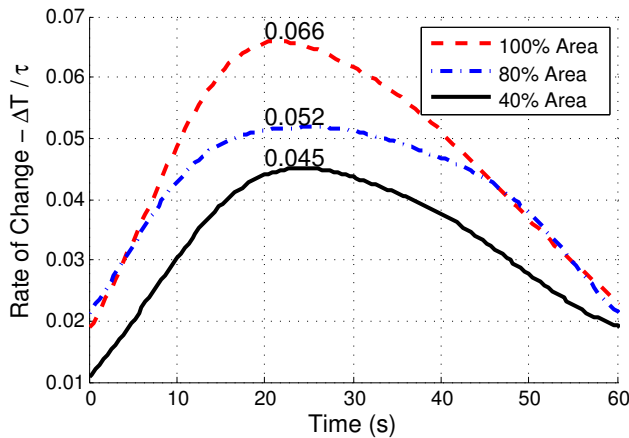
Figure 20: Temperature change rate for varying contact areas.
