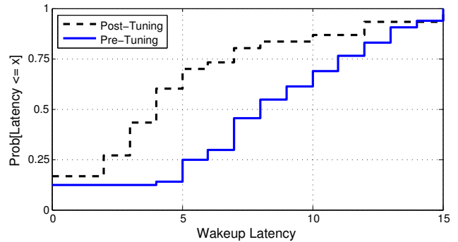
Figure 15: CDF of wakeup latency for a single node before and after tuning the wakeup threshold.
