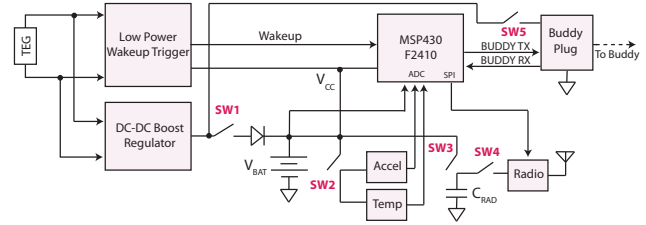
Figure 4: DoubleDip circuitry, including low power wakeup, RF, accelerometer, buddy plug for energy transfer, temperature sensors, and analog switches for power-gating and duty cycling.
