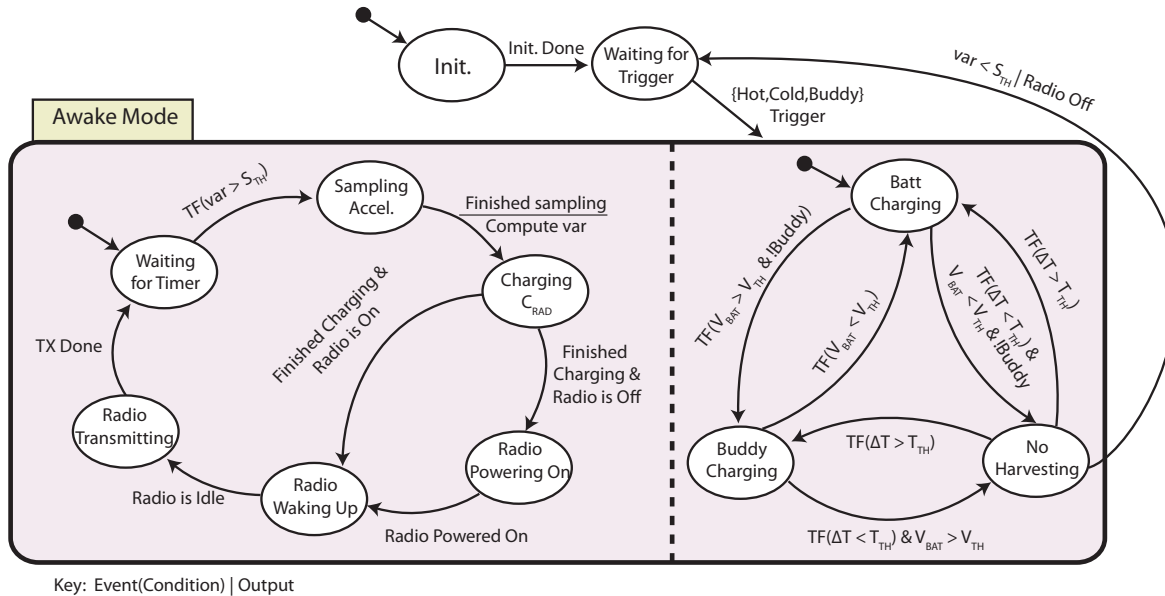
Figure 6: DoubleDip state chart, showing conditions for entering and exiting harvesting modes, buddy harvesting, sensing and relaying acceleration variance, and returning to low power wakeup. Events specified as TF are Timer Fired events. The dashed line within awake mode indicates concurrency.
