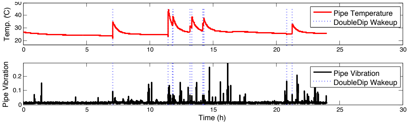
Figure 1: Sample data of pipe temperature, wakeup triggers from DoubleDip, and pipe vibration. Spurious vibrations would cause frequent false wakeups with vibration-based LPL even though water use is sporadic.
