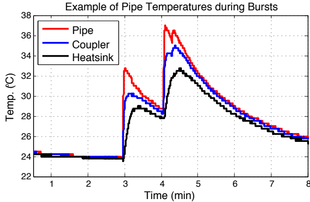
Figure 19: Example temperature curves for hot water bursts, showing the difference between T_{Pipe} and T_{Coupler} as well as the non-ideality of the heatsink.
