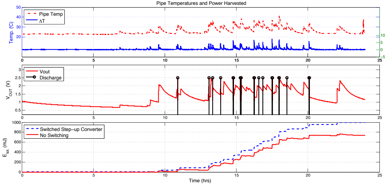
Figure 11: Power harvested for an example weekday during March (24 hours starting at 12:00am). From top to bottom, plots show (1) Pipe temperature and \Delta T = T_{coupler} - T_{heatsink} ; (2) output voltage across a 15 mF capacitor with discharge signals when the capacitor gets close to saturation; and (3) cumulative energy harvested over the entire day, in mJ. Cumulative energy is shown when the step-up DC-DC converter is always on and when it is switched on an as-needed basis.
