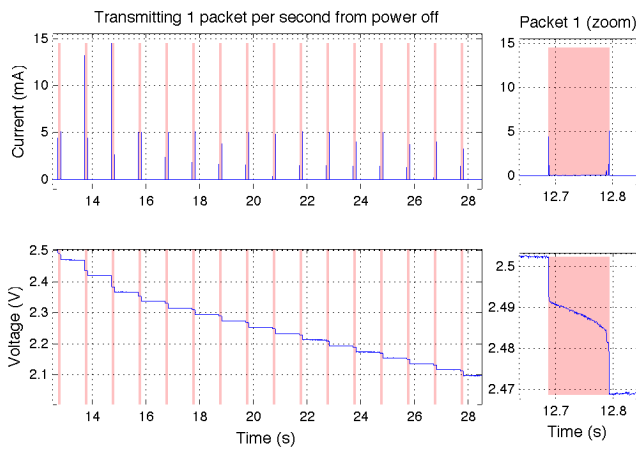
Figure 17: Current consumption of a Nordic nRF24L01+ radio operating from a capacitor. The radio sends one 32 Byte packet every second and then is turned off (power-gated). The right-most plot shows a zoomed in version of what occurs to the voltage across the transient capacitor during a single transmission.
