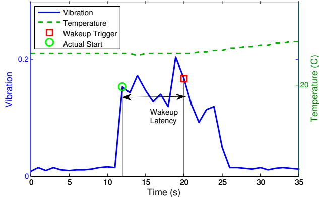
Figure 13: Example calculation of wakeup latency. The green circle indicates the start of the water event, as determined by the vibration variance (y-axis). The red square indicates the time the wakeup trigger fired. The difference between these two is the latency.
