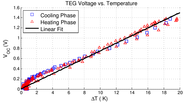
Figure 7: Open circuit output voltage for a CUI60333 Peltier module vs. differential temperature across the ceramic plates. The relationship is approximately linear, as per the physics governing the effect. For the heating and cooling phase, r^2 = 98.9 and 95.8 , respectively.
