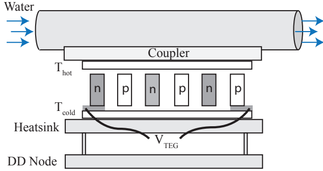
Figure 2: Diagram of DD node attached to water pipe, showing coupler, Peltier, heatsink, and the node itself.
