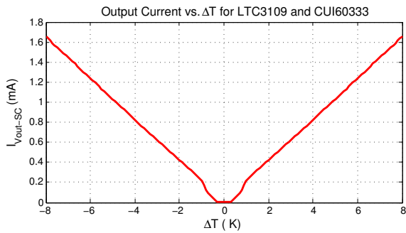
Figure 8: Short circuit output current of boost regulator vs. input temperature differential, \Delta T .
