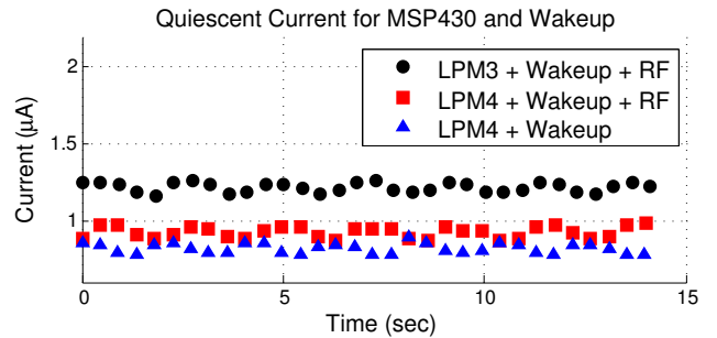
Figure 12: Current consumption for low power wakeup circuitry and deep sleep MSP430 (LPM4). Current is shown with and without SPI pins configured for RF and compared to a sleep mode with low power clock (LPM3).
