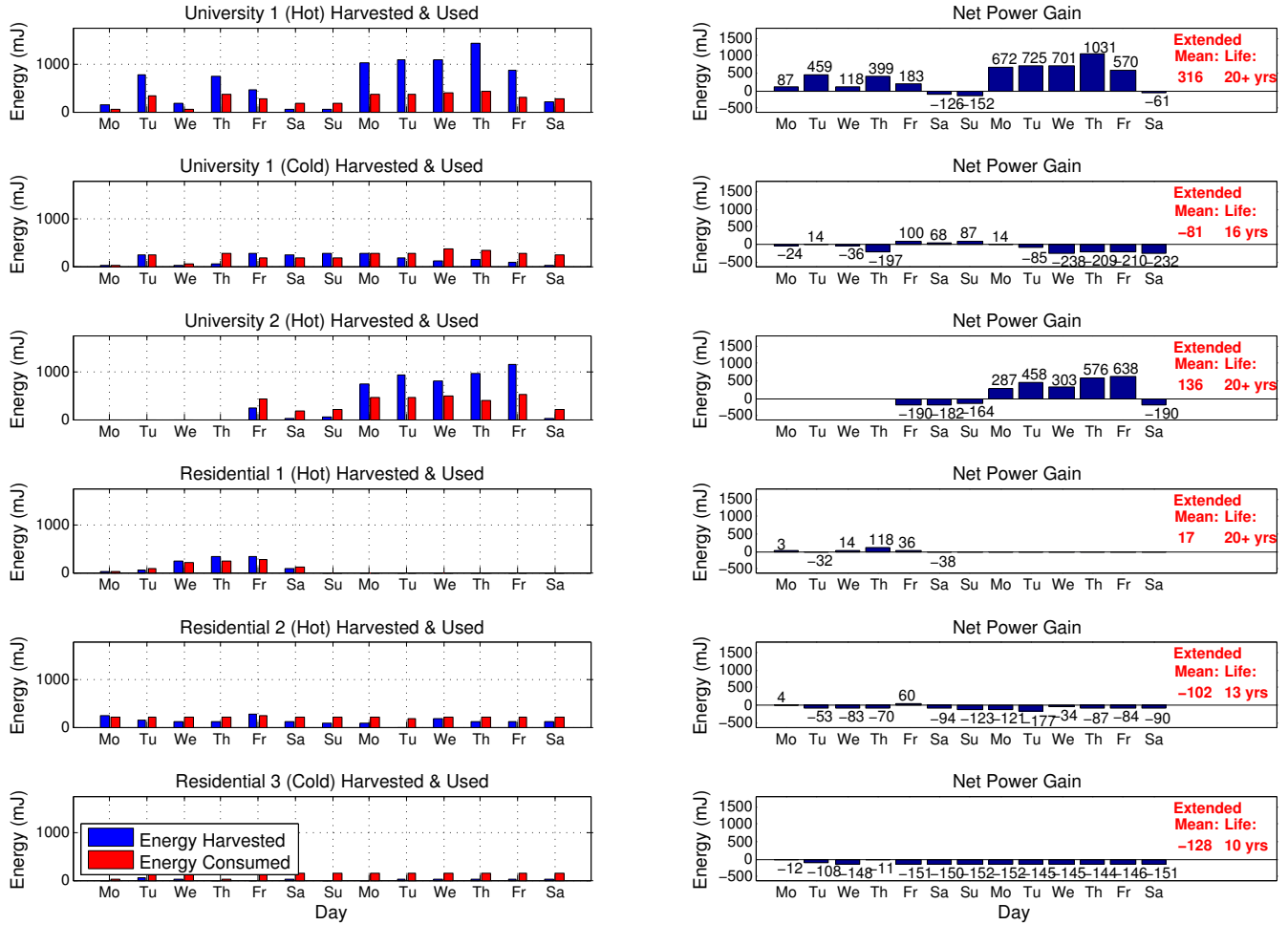
Figure 18: Energy harvested and consumed per day for 2 example weeks. By subtracting energy consumed from energy harvested (left) we get the net energy per day (right). Mean daily energy and lifetime estimates are calculated using the entire data set for each node (not shown). University 1 (Hot), University 2 (Hot), and Residential 1(Hot) show a net positive in energy gained, indicating that the node lifetime is limited only by the battery shelf life. The others (while suffering a net loss in energy) are still considerably better than they would have been had the same circuitry been used without harvesting.
