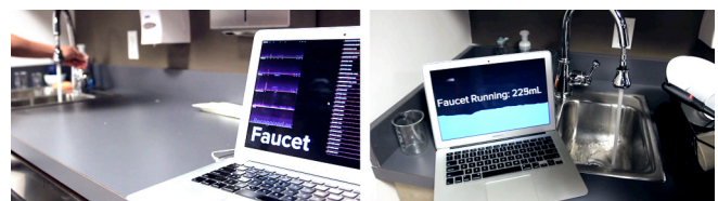
Figure 17. A first-order “faucet running” synthetic sensor (left) can be used to power a second-order “water volume” synthetic sensor (right).
