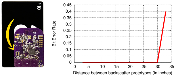
Figure 17—BER for communication between two cards with integrated antennas. Amazon card shown for comparison.
