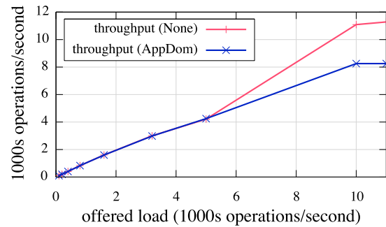
Figure 10: Operation invocation throughput as a function of offered load with and without Application Domain isolation
