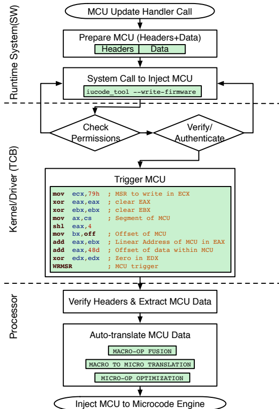
Figure 2: Auto-translation Procedure
