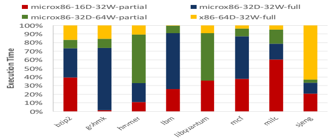
Figure 13. Execution Time Breakdown on the best composite-ISA CMP optimized for Multi-programmed Throughput under 48mm 2 Area Budget most applications migrate to a core with a different feature set at least once. Fourth, the benchmark hammer that exhibits significant register pressure tends to always execute on a feature set with a register depth of 64. Interestingly, we found that phases with considerable irregular branch activity, due to indirect branches and function pointer calls, prefer full predication since it eases the pressure on the branch predictor by converting some of the control flow into data flow. This is evidenced by the benchmarks sjeng and gobmk .
